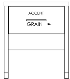
FG-C604 Nightstand...20 x 18 x 28 FG-C604A Nightstand...24 x 18 x 28
