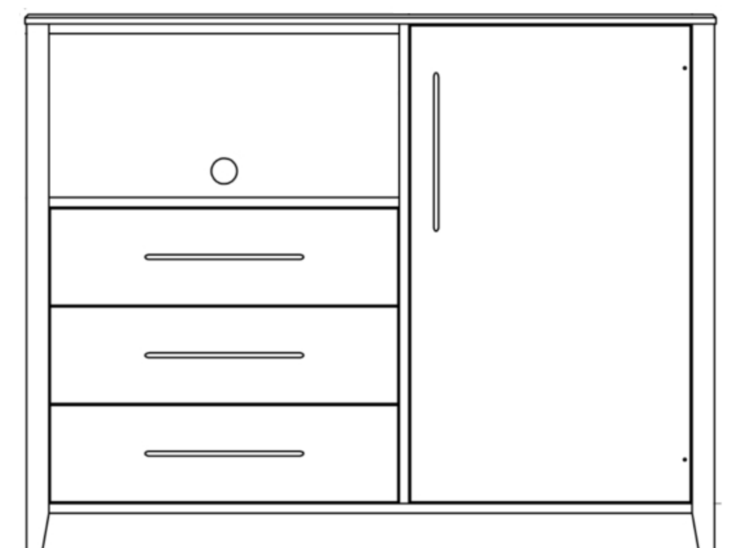
TG-M0823A Microfridge w/Door 54 x 24 x 42 Microwave Opening: 27 3/8 W x 21 3/8 D x 12 13/16 H Microfridge Opening: 22 1/8 W x 21 3/8 D x 36 3/4 H
