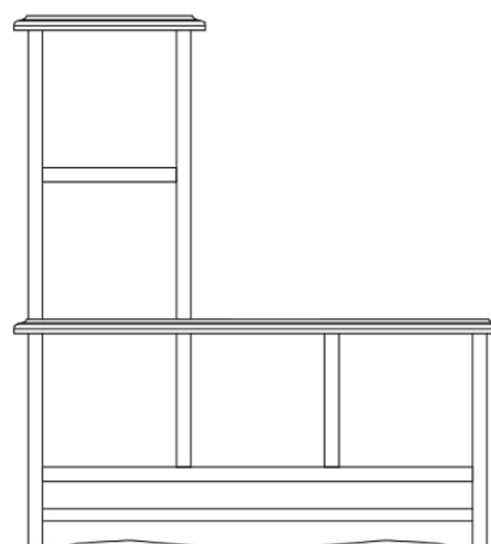
SI-B535D Towel Shelf (L) 25 1/2 x 8 x 27 7/8
