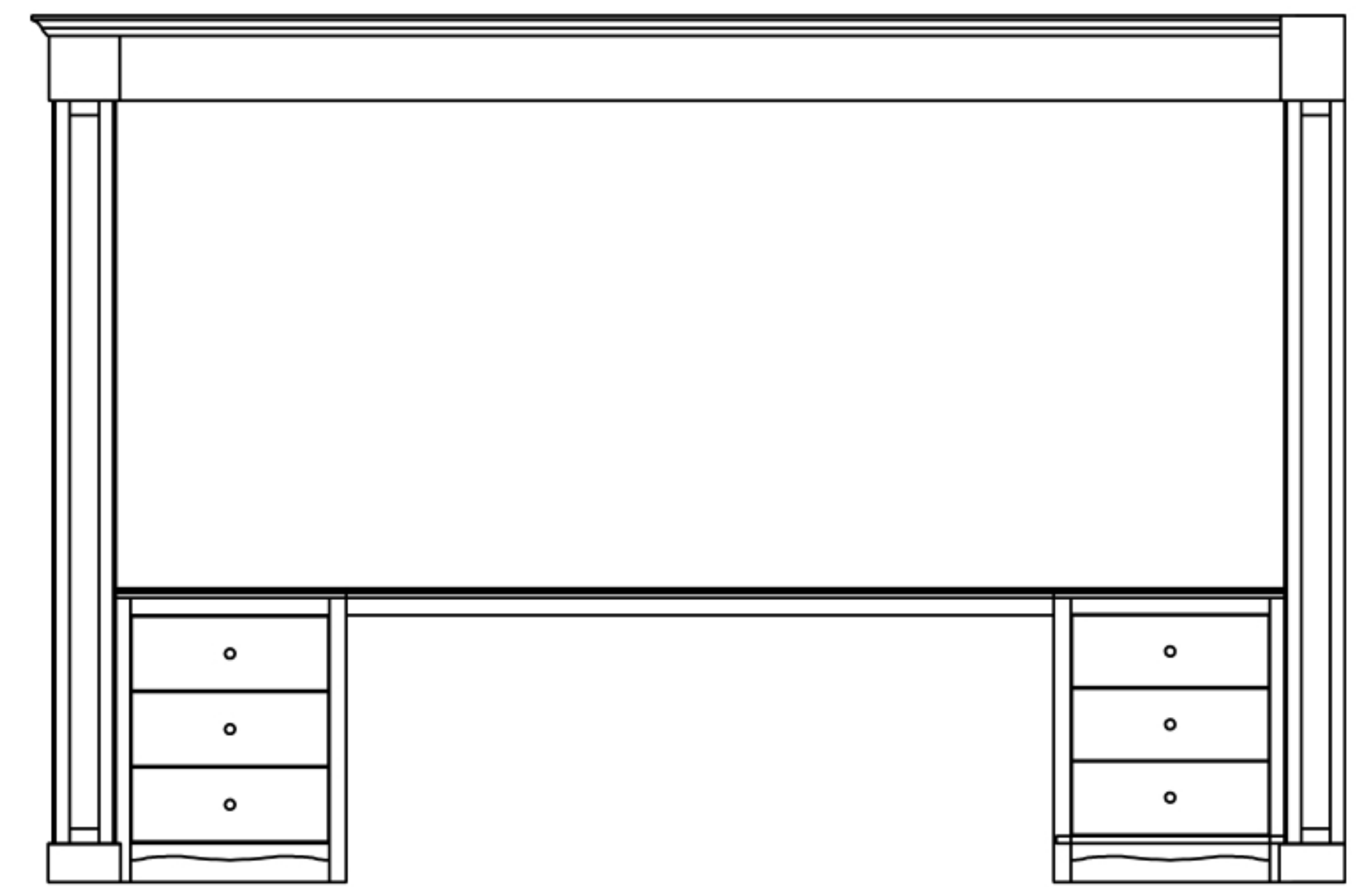
SI-B535 Suite Divider w/Canopy 135 5/16 x 34 x 89 1/4 SI-B535A Suite Divider w/Canopy 123 5/16 x 34 x 89 1/4 SI-B535B Suite Divider w/Canopy 135 5/16 x 44 1/2 x 89 1/4
