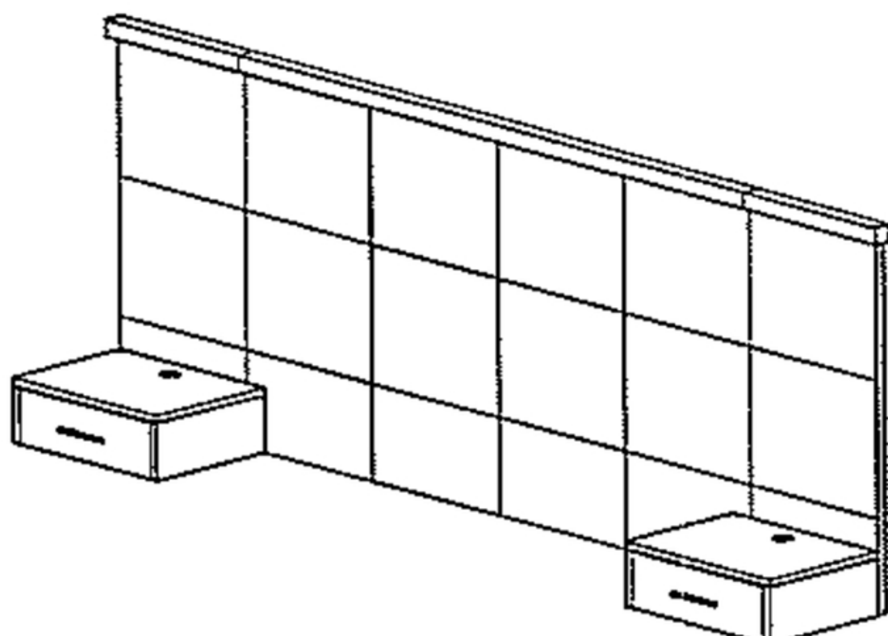
SG-209 (VPCS) 120" NS-I611R Queen Headboard (G-202) 120 x 19 1/2 x 48
