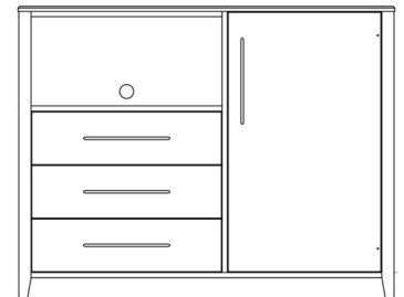
TG-0823G Microfridge.....54 x 22 x 42 Microwave Opening: 27 3/8 W x 21 3/8 D x 12 13/16 H Microfridge Opening: 22 1/8 W x 21 3/8 D x 36 3/4 H TG-0823R Microfridge w/Door...54 x 24 x 42 Microwave Opening: 27 3/8 W x 21 7/8 D x 12 13/16 H Microfridge Opening: 22 1/8 W x 21 7/8 D x 37 1/2 H
