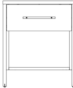
TY-I204 King Nightstand.....22 x 18 x 26 TY-I204A Queen/Dbl Nightstand...24 x 18 x 26
