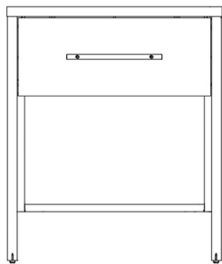
TY-S204 King Nightstand...20 x 18 x 26 TY-S204A Queen Nightstand...24 x 18 x 26
